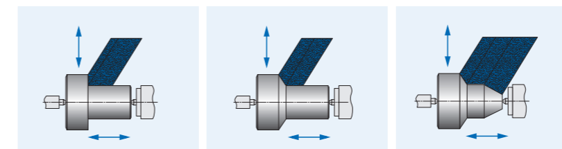
EXTERNAL ANGULAR PLUNGE GRINDING WITH EJ 11, EJ 31 AND EJ 51
